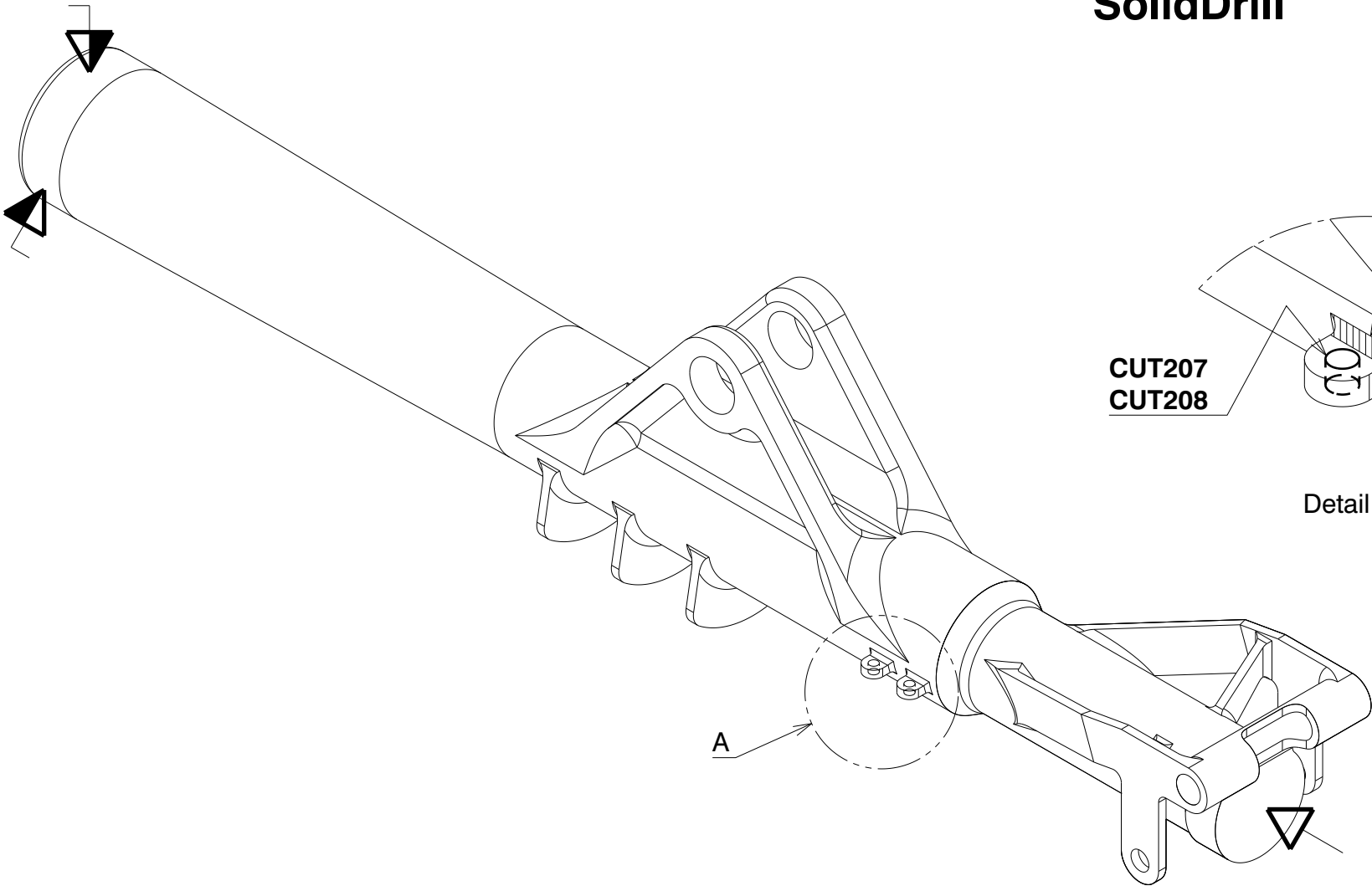
Isometric view
