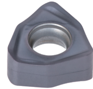
WXMU03-MM Economical double-sided inserts with six cutting edges
