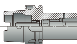
HSK-63A
