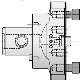
Bridge adaptor
