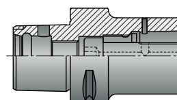
Reduction adaptor
