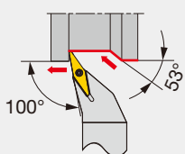
Cutting edge style H
