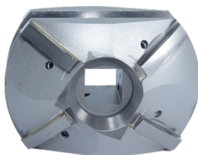
Sphere shape cutter & Slot cutter
