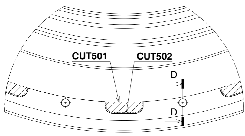
Auxiliary view B Scale: 1:3
