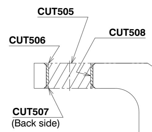
Section cut D-D Scale: 2:1
