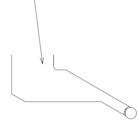
Special Tool AH8000
