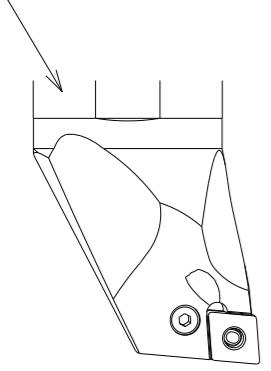
StreamJetBar AH8000
