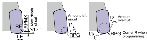
Max. depth of cut APMX (mm) Corner radius RE (mm) LE (mm) Corner R when programming RPG Amount left uncut t1 (mm) Amount overcut t2 (mm) 1 1.2 3 1 0.6 - 1 1.2 3 1.5 0.5 - 1 1.2 3 2 0.25 0.08 1 1.2 3 2.5 0.14 0.26
