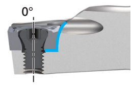
Conventional (CCMT060204...for boring bar)
