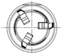
3 teeth, Cutter diameters: ø20.5 mm and ø22.0 mm
