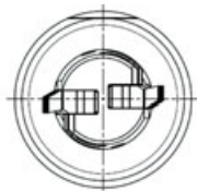
2 teeth, Cutter diameters: ø0.6693" and ø0.7480" (ø17 mm and ø19 mm)
