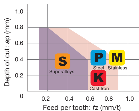
TungRec 07 type HJ inserts Standard conditions
