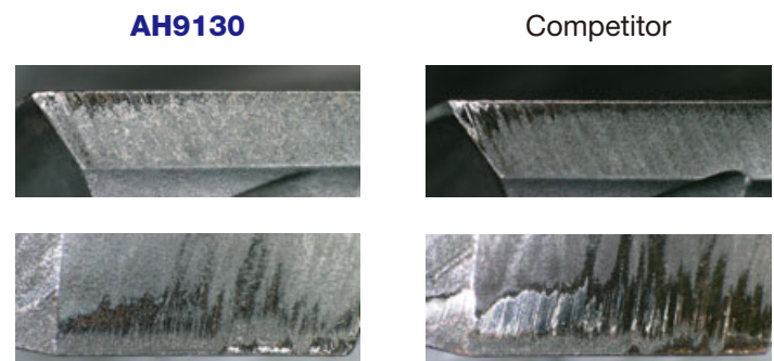
■ Edge damage after 100 m machined
