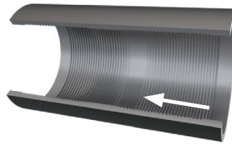
API standard buttress thread
