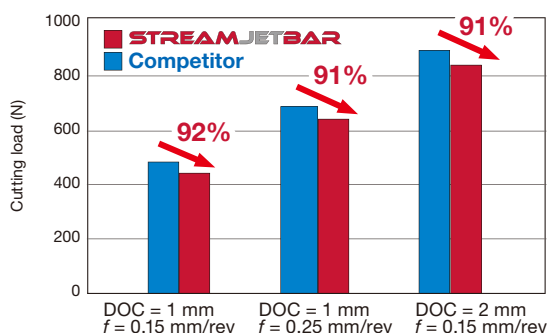
Cutting load comparison
