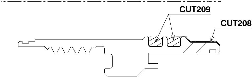
Section cut H-H
