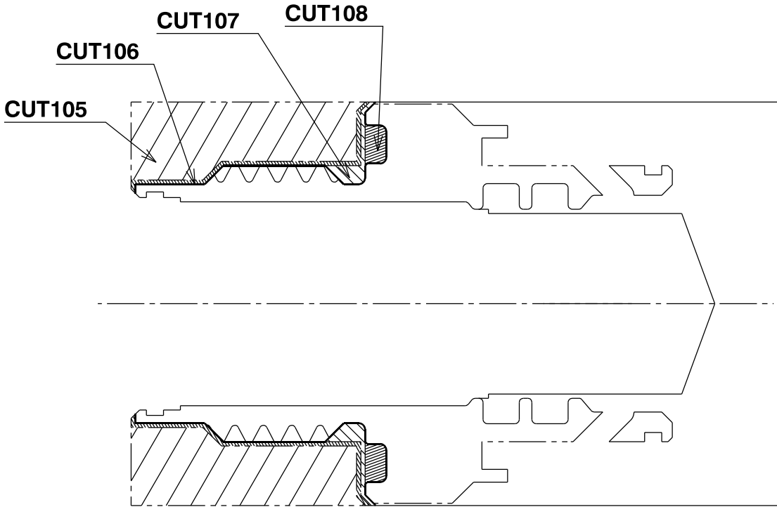
Section cut C-C
