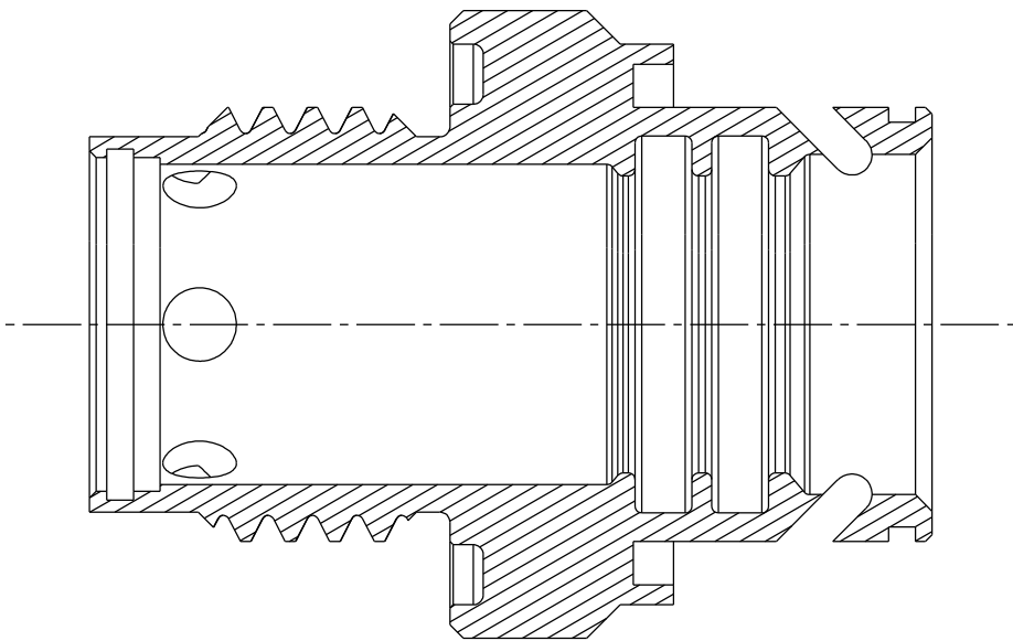
Section view A-A
