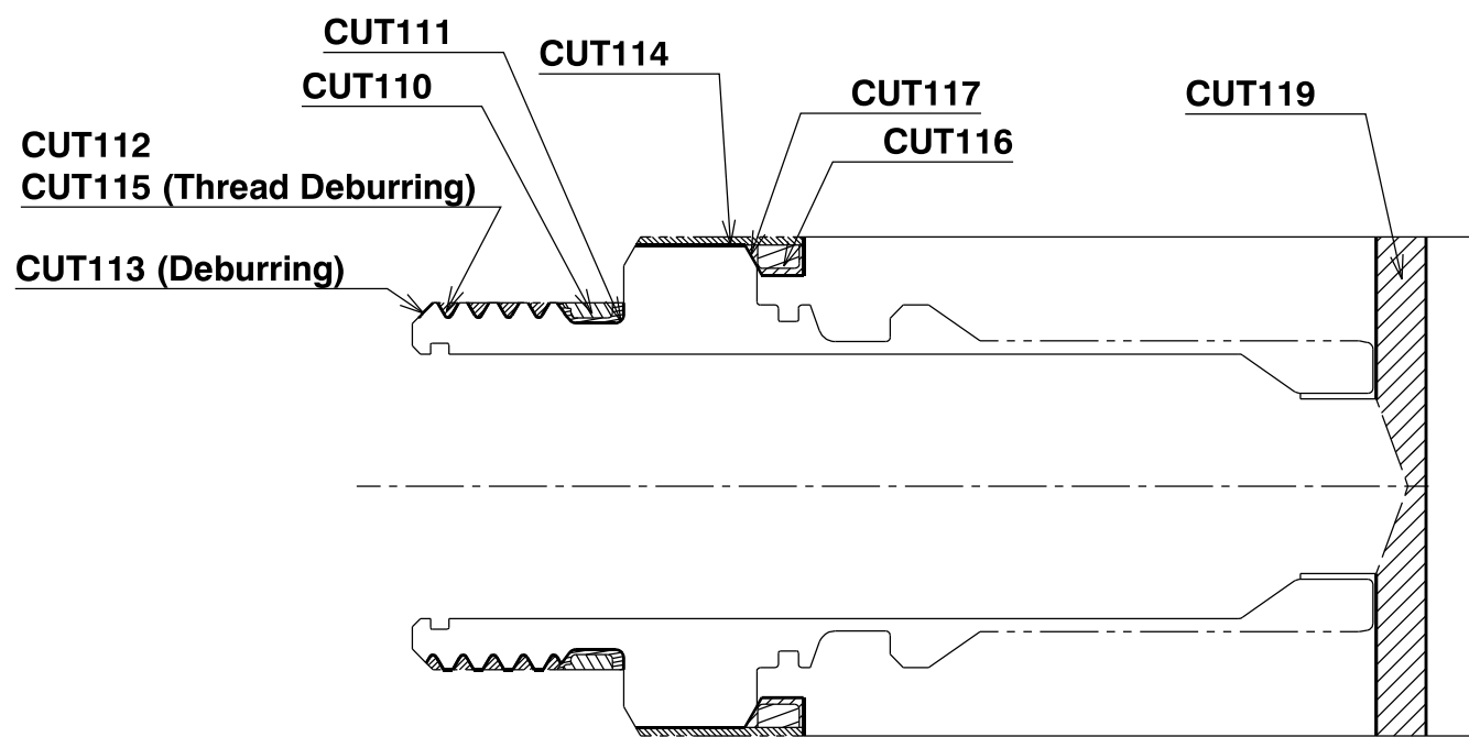
Section cut F-F
