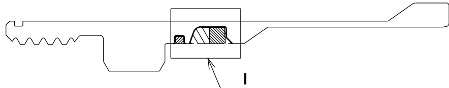
Section cut H-H
