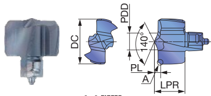
ADAM DRILL DMF040 - DMF059
